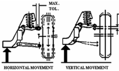
SPRING ON UPPER CONTROL ARM
